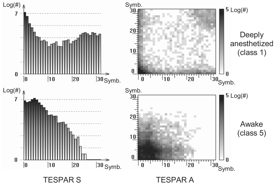
Fig. 2. TESPAR S and A matrices ( L = 1 ) for awake (class 5) and deeply anesthetized states (class 1). The S matrix counts how many times symbols appear in the data stream. The A matrix represents in a gray scale the number of occurrences for each symbol pair situated L symbols apart. The log transformation (see section 2.5 “Feature extraction, TESPAR”) has been applied to the matrices. Prominent differences can be seen in the matrices for the two extreme states (awake, deeply anesthetized).
