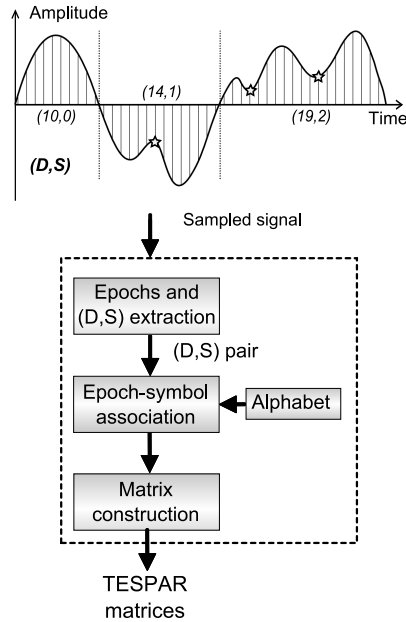
Fig. 1. TESPAP coding diagram block. It shows how the digital signal is divided in epochs (delimited by vertical dotted lines). Each epoch is characterized by its number of samples ( D ) and its number of local minima ( S ) (we refer to the local minima of the absolute value of the waveform). The (D, S) pair stream (values showed for each epoch) is then transformed in a symbol stream, with the help of an alphabet that maps each pair onto a symbol (number). The symbol stream is further condensed in TESPAP A or S matrices in the final stage of the coder.
