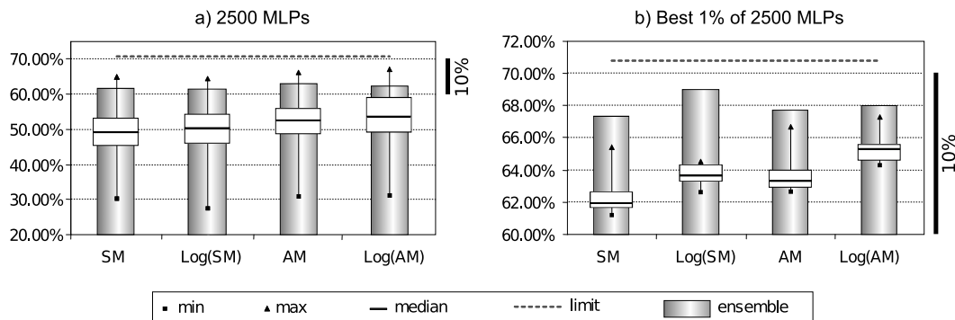
Fig. 3. The classification performance of the four sets of 2500 MLP networks (a) and the selection of the best 1% (b). On the X axis we indicate which TESP matrix is used and whether the log nonlinearity is applied or not. The dotted line represents the self-consistency of the human classifier, which is taken as the maximum achievable performance by the artificial classifier. The box plots show, for each distribution, the median, the quartiles q_1 and q_3 , and the minimum and the maximum performances. The ensemble performance is presented through thick grey bars. Note the different scales in a) and b) that are emphasized by the 10% indication (thick black bars shown on the right).
